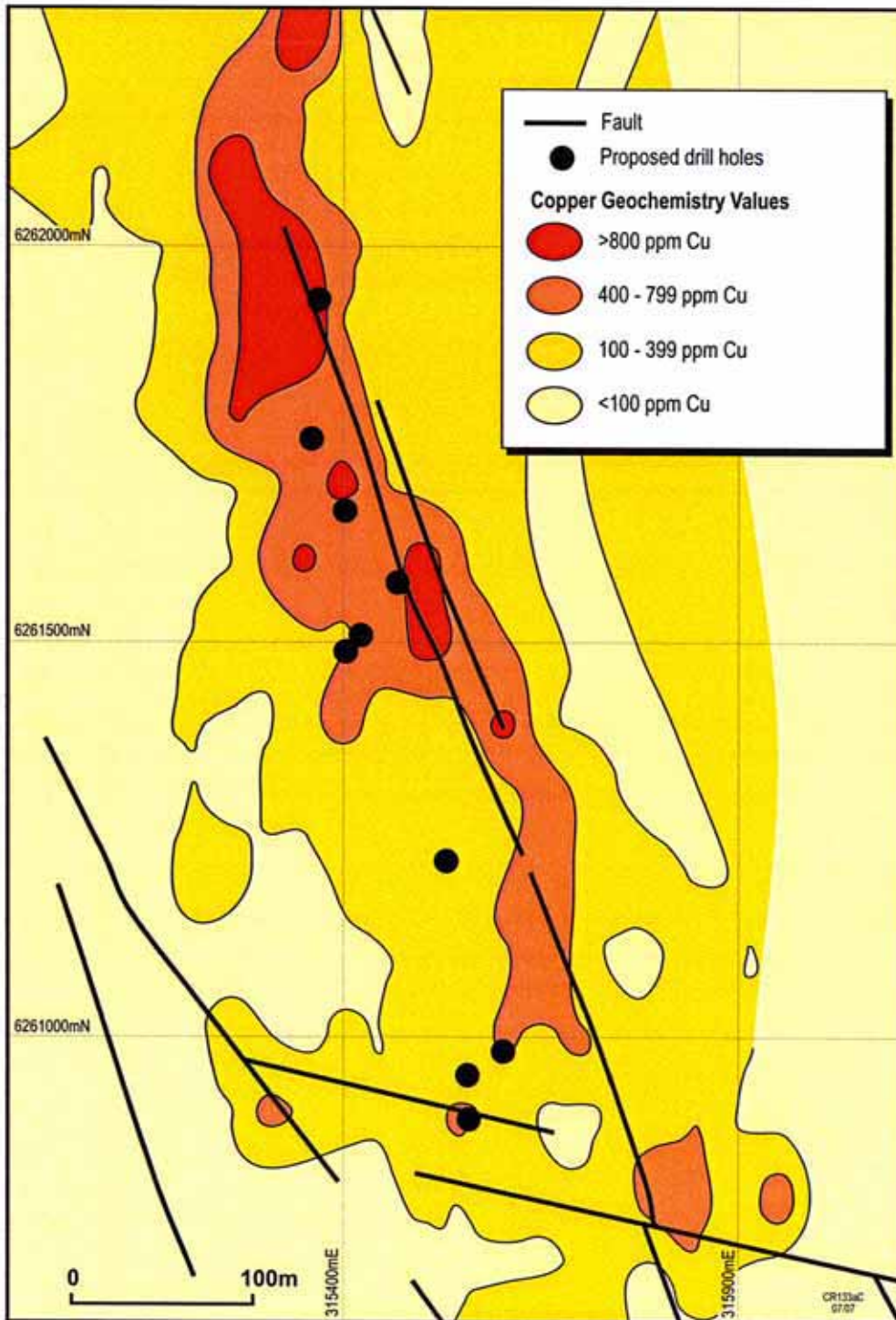
COPPER GEOCHEMISTRY OF PRINCESS ROYAL PROSPECT AREA
