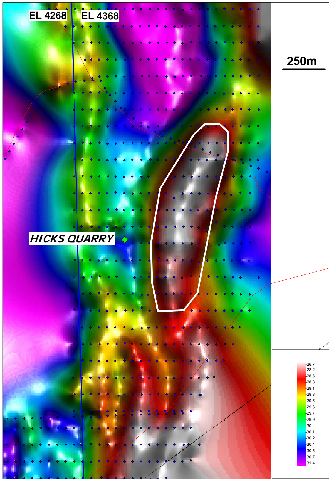
Figure 1 – Hicks Prospect Gravity Anomaly
